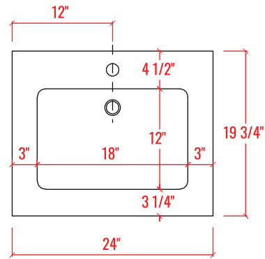
ELEVATION VIEW
